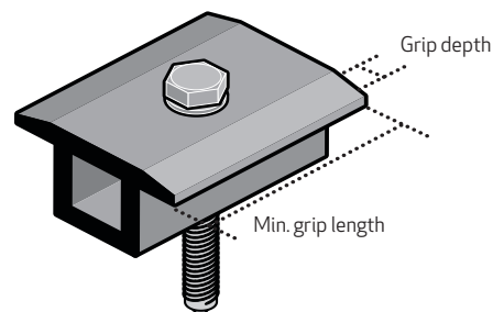
Fig. 1: Clamp specifications
