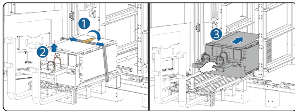
Figure 4-10 Installing the battery pack in the ESS
