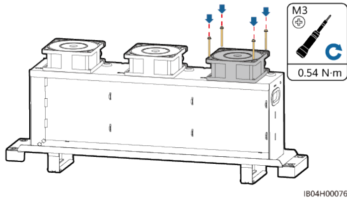
Figure 9-8 Installing a fan
