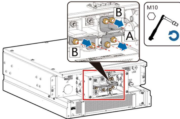
Figure 8-5 Removing short-circuiting copper bars (97 kWh/129 kWh/161 kWh model)
