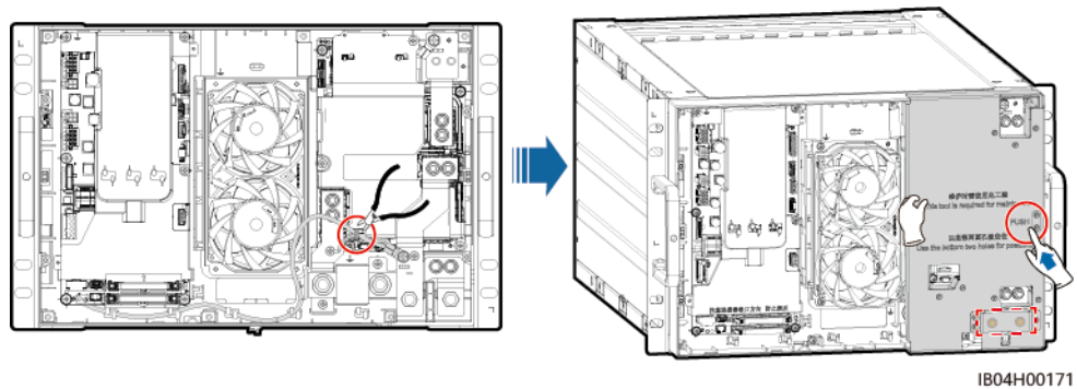
Figure 5-5 Installing the battery pack fixture
