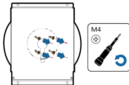
Figure 10-6 Removing the internal fan
