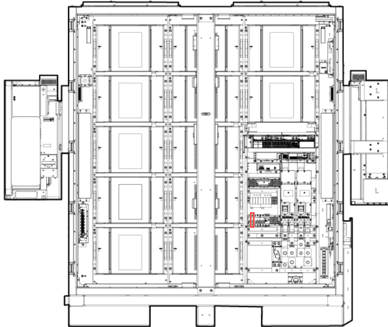
Figure 13-6 Position of the switch
