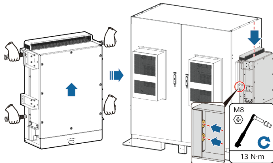
Figure 8-12 Installing the rack controller
