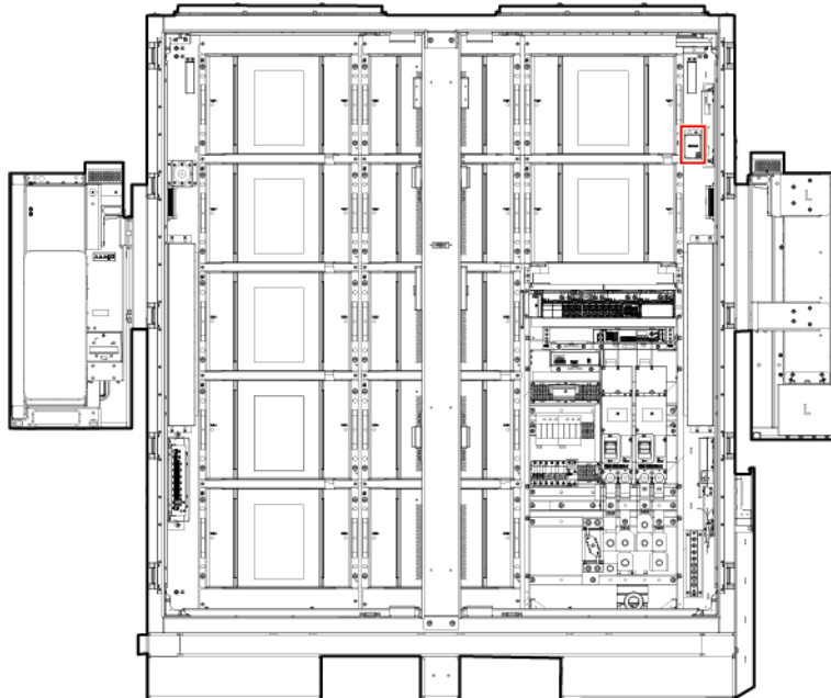
Figure 21-1 Position of the T/H sensor
