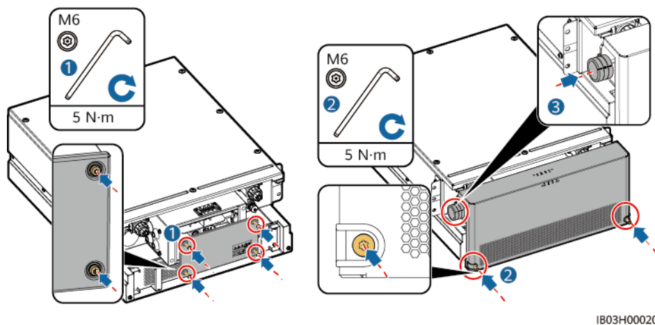
Figure 8-17 Installing covers
