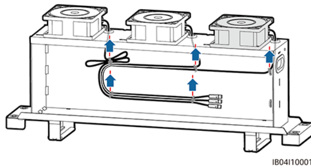
Figure 9-4 Removing the FAN 1 cable ties
