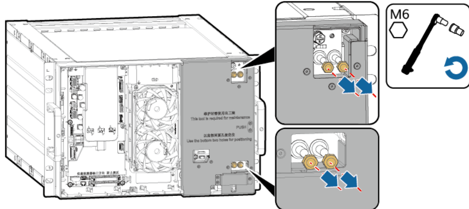
Figure 5-6 Removing the nuts
