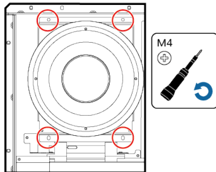
Figure 10-4 Removing the internal fan and the fixing plate
