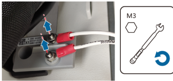
Figure 20-2 Removing the water sensor
