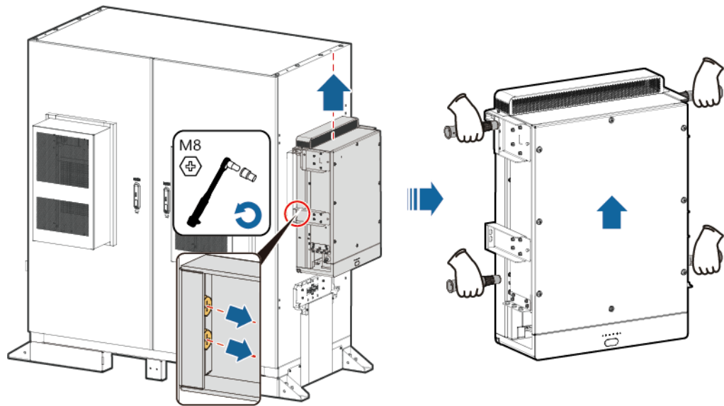
Figure 8-9 Removing the rack controller
