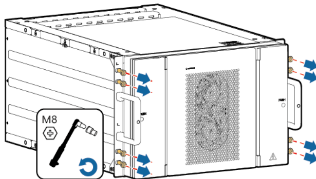
Figure 4-3 Removing screws
