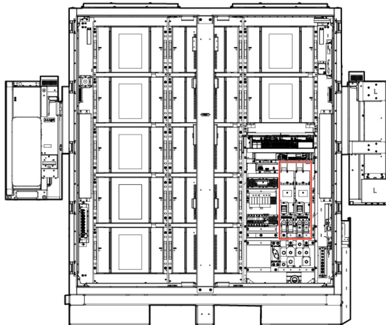
Figure 13-1 Position of the DC switch
