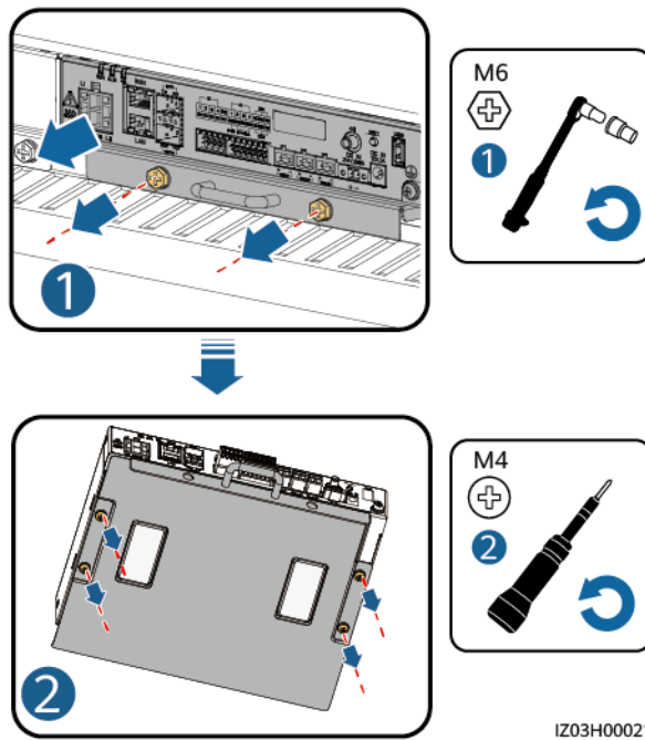
Figure 18-3 Removing the faulty CMU
