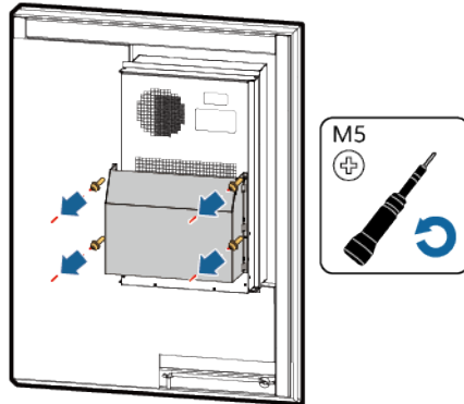
Figure 10-10 Removing the air duct
