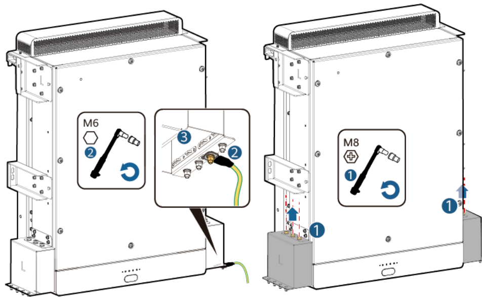
Figure 8-7 Removing the ground cable and protective covers
