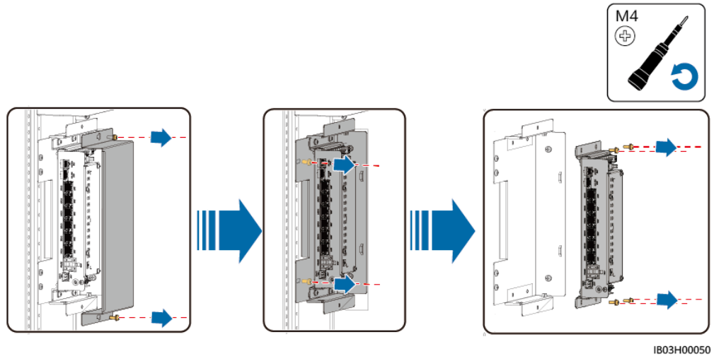
Figure 27-2 Removing the I/O expansion board
