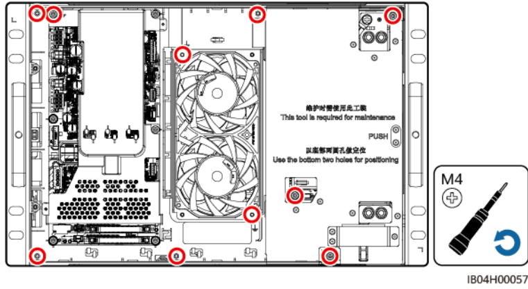
Figure 5-7 Removing the screws
