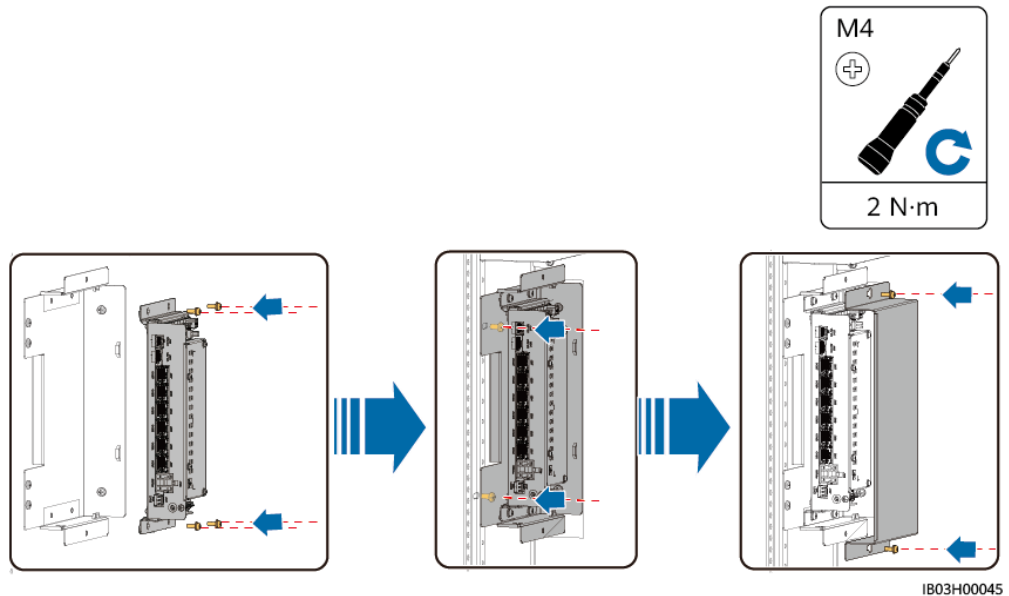
Figure 27-3 Installing an I/O expansion board
