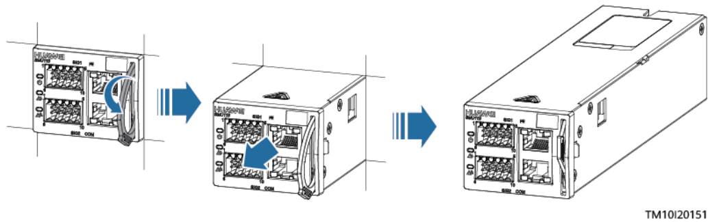
Figure 25-2 Removing the old SMU
