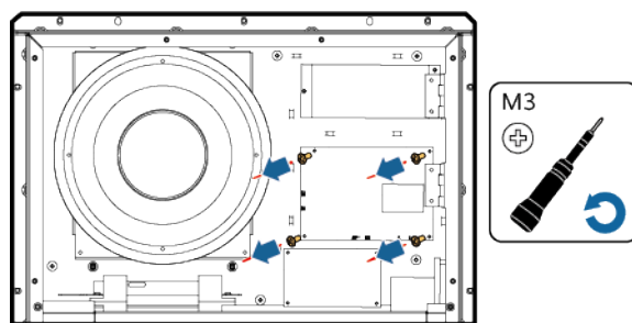
Figure 10-13 Removing the main control board
