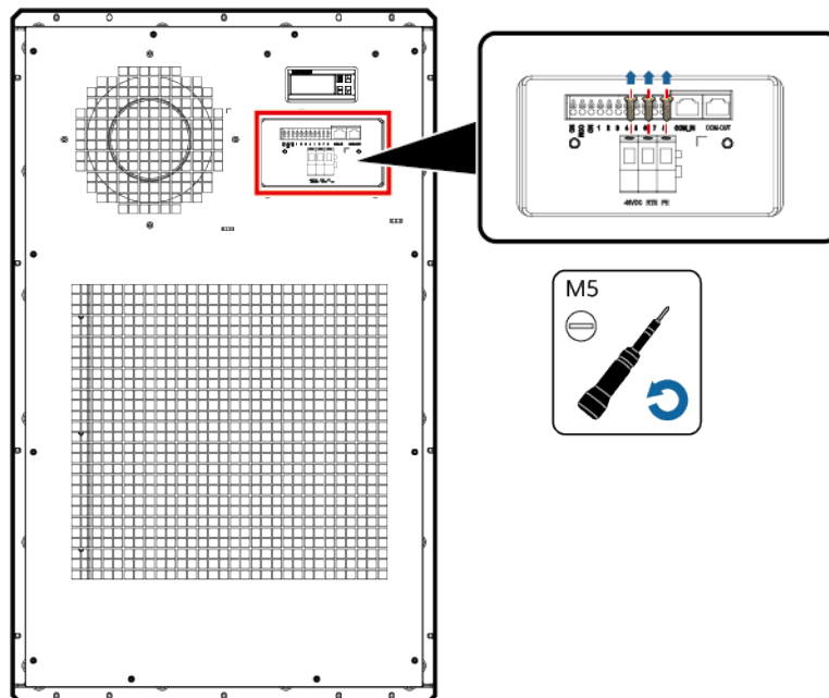
Figure 10-11 Removing air conditioner cables
