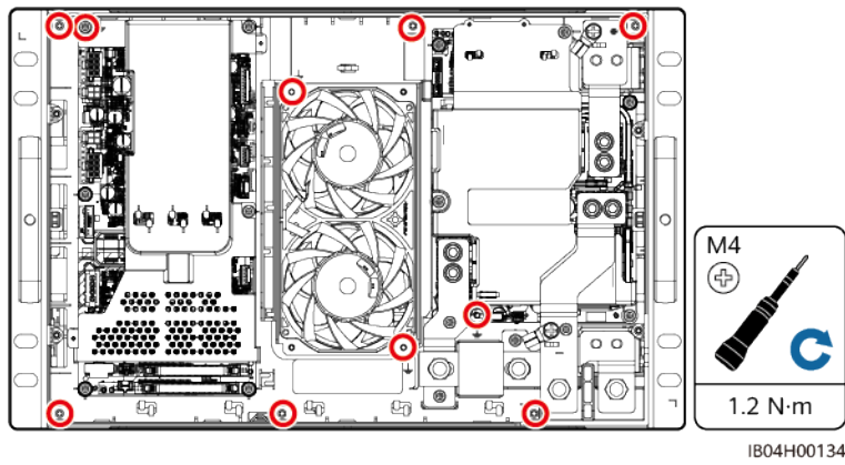
Figure 5-8 Installing the screws
