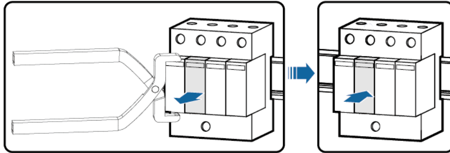
Figure 14-2 Replacing a surge protection module
