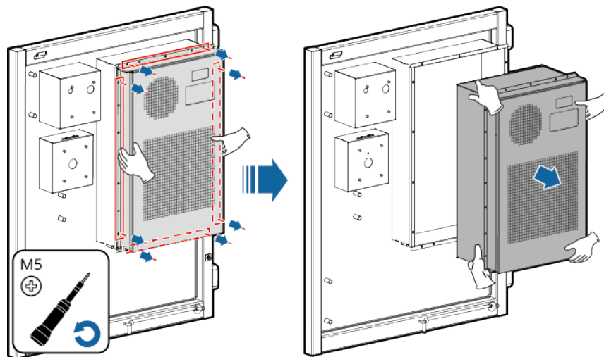
Figure 10-18 Removing the old air conditioner
