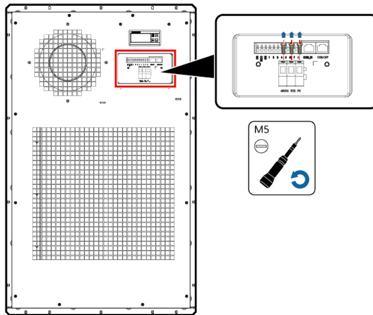
Figure 10-17 Removing air conditioner cables
