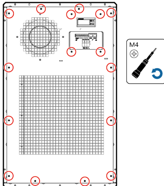
Figure 10-3 Removing the front cover of the air conditioner
