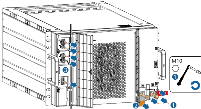
Figure 4-2 Removing copper bars and cables
