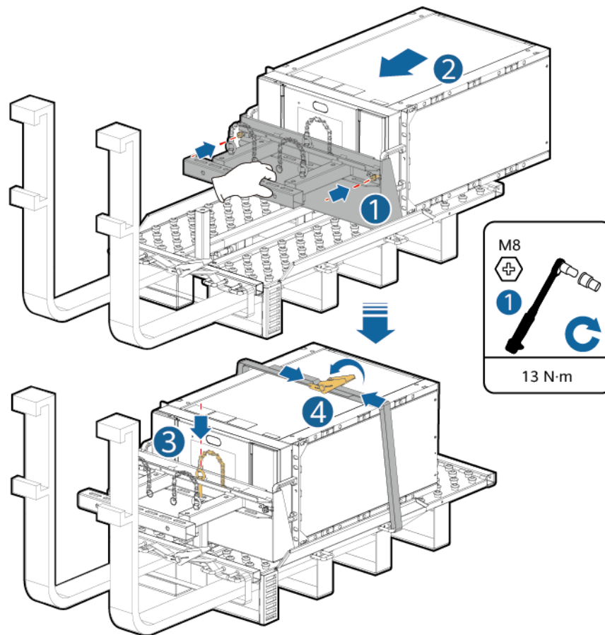
Figure 4-7 Securing the battery pack
