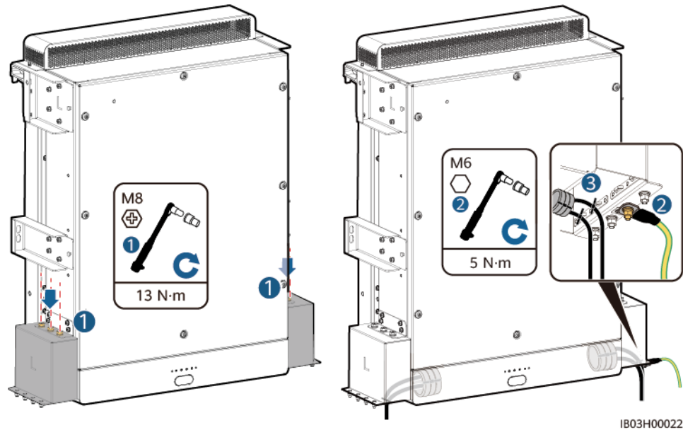
Figure 8-18 Connecting the ground cable
