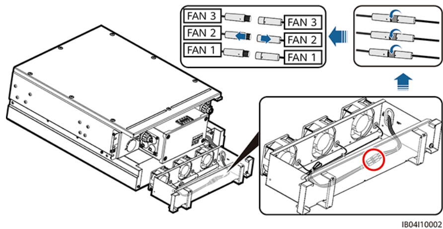
Figure 9-3 Disconnecting cables
