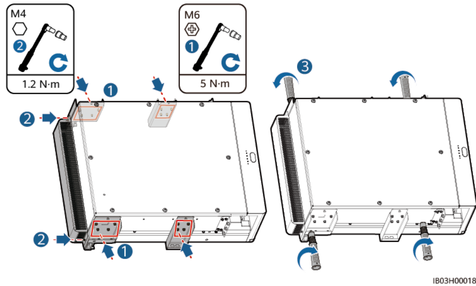
Figure 8-11 Installing mounting kits
