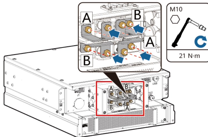
Figure 8-13 Installing short-circuiting copper bars (200 kWh model)
