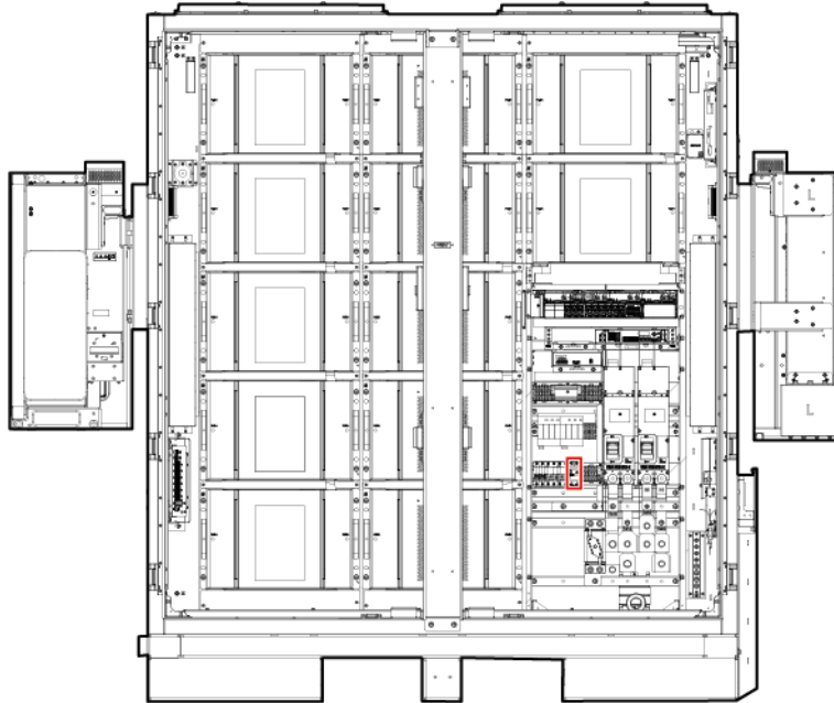
Figure 13-5 Position of the switch
