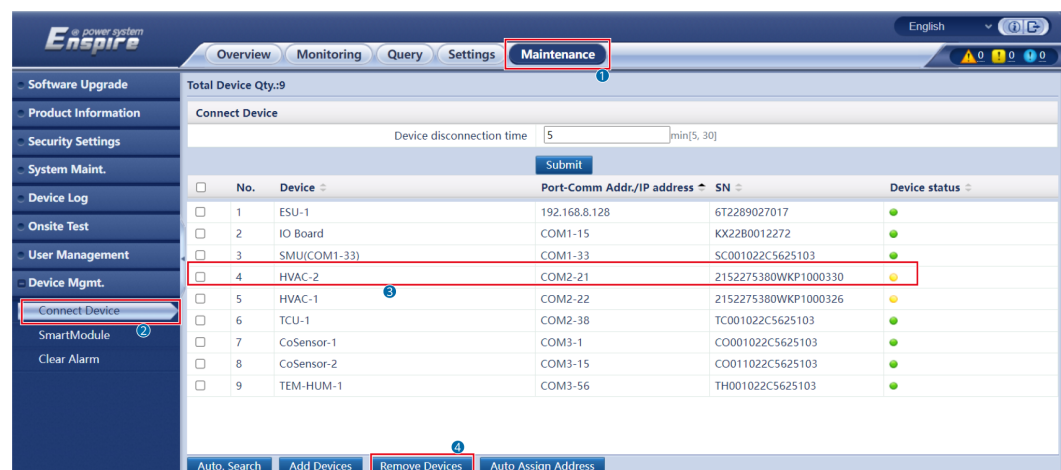
Figure 10-20 Removing the old air conditioner
