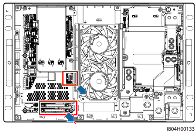
Figure 5-4 Removing the flat cables
