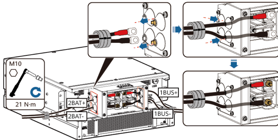
Figure 8-15 Installing cables (part 1)
