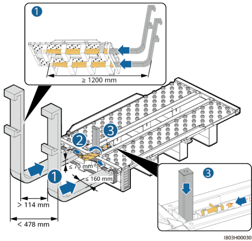
Figure 4-6 Assembling the installation kit
