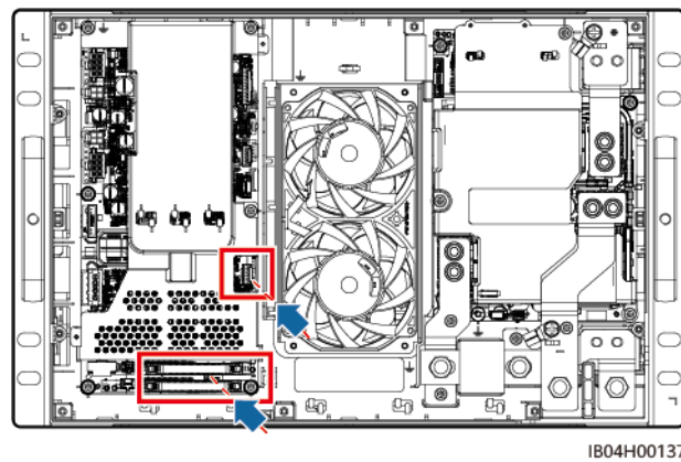
Figure 5-11 Installing the flat cables
