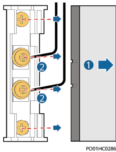
Figure 19-2 Removing the door status sensor
