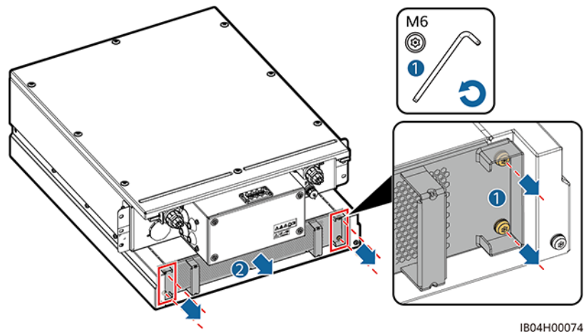
Figure 9-2 Pulling out the fan tray
