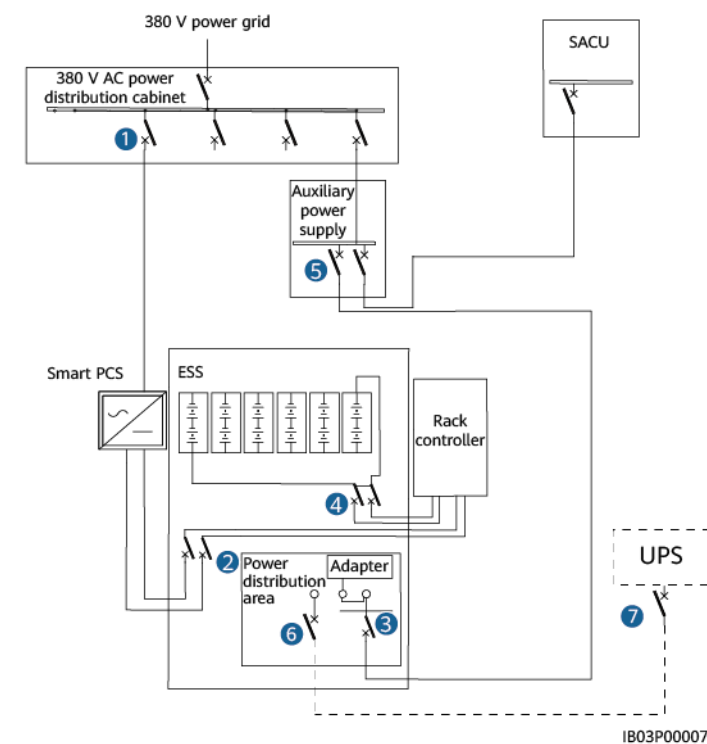
Figure 2-2 Power-off process
