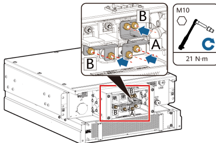
Figure 8-14 Installing short-circuiting copper bars (97 kWh/129 kWh/161 kWh model)
