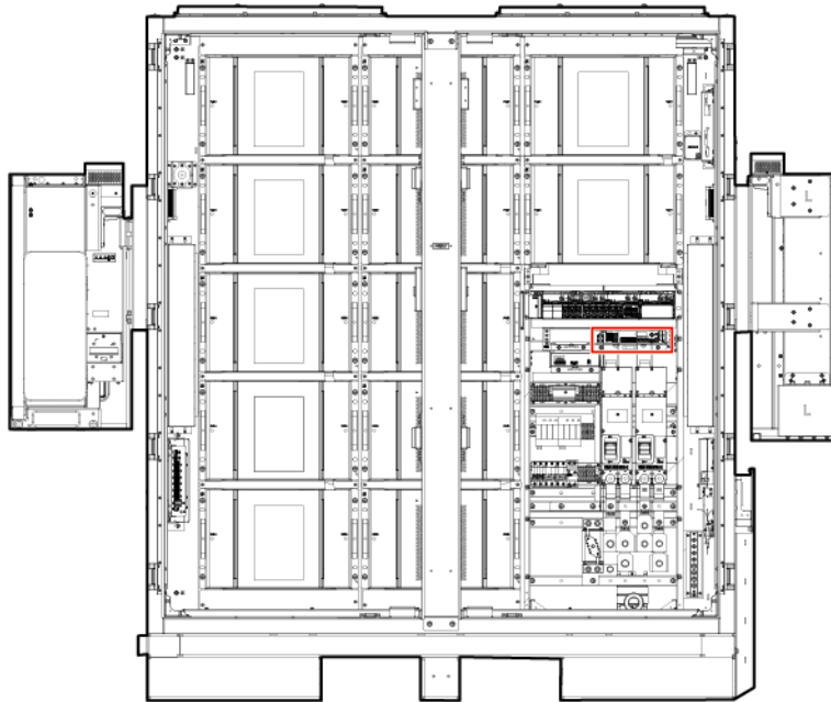
Figure 18-1 Position of the CMU
