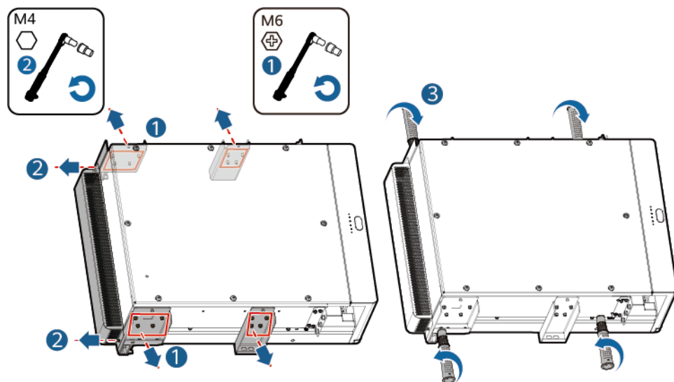
Figure 8-10 Removing mounting kits
