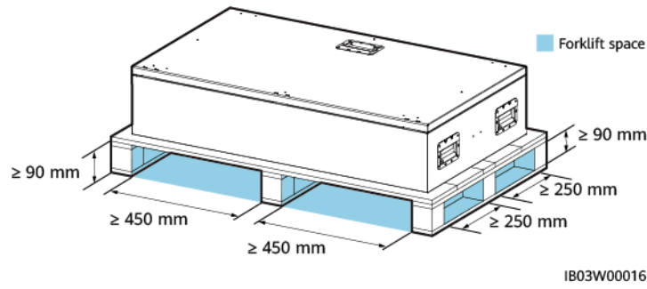
Figure 4-4 Forklift space dimensions
