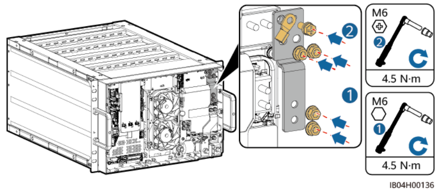
Figure 5-10 Installing the short copper bar
