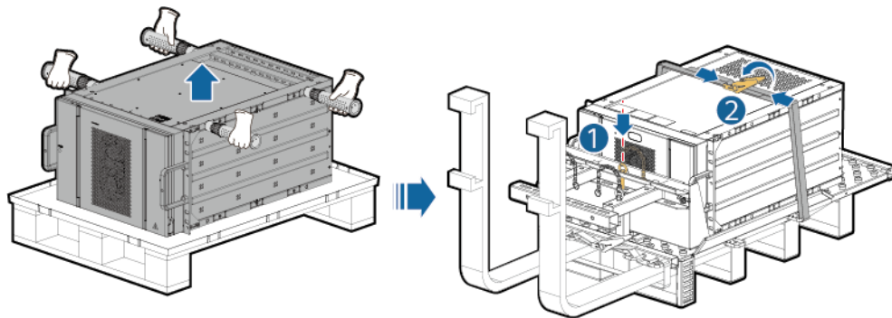
Figure 4-9 Moving the new battery onto the installation kit
