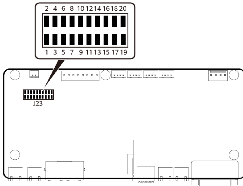
Figure 22-4 Positions of the jumpers on the TCUE control board
