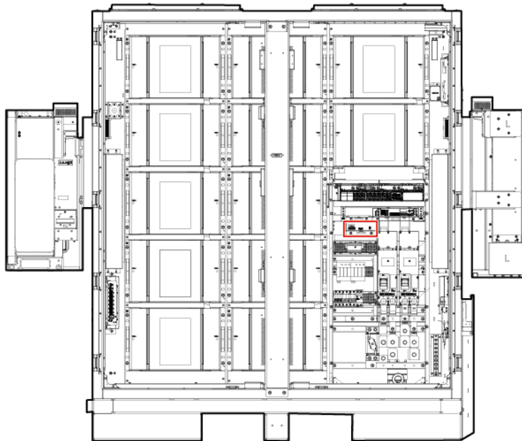
Figure 17-1 Position of the CMU adapter
