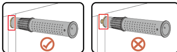
Figure 8-8 Correct and incorrect lifting handle installation
