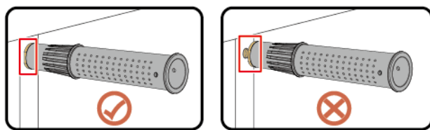
Figure 4-8 Correct and incorrect lifting handle installation
