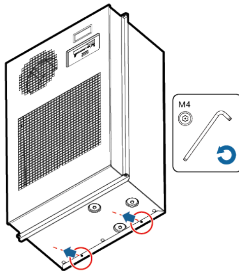
Figure 10-7 Removing security torx screws
