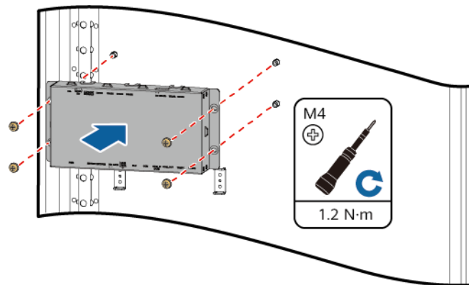
Figure 22-6 Reinstalling the TCUE control box
