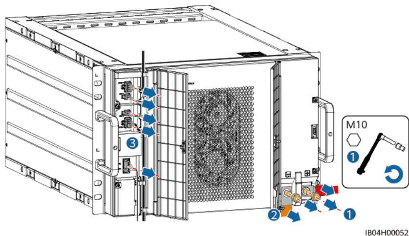
Figure 5-2 Removing copper bars and cables
