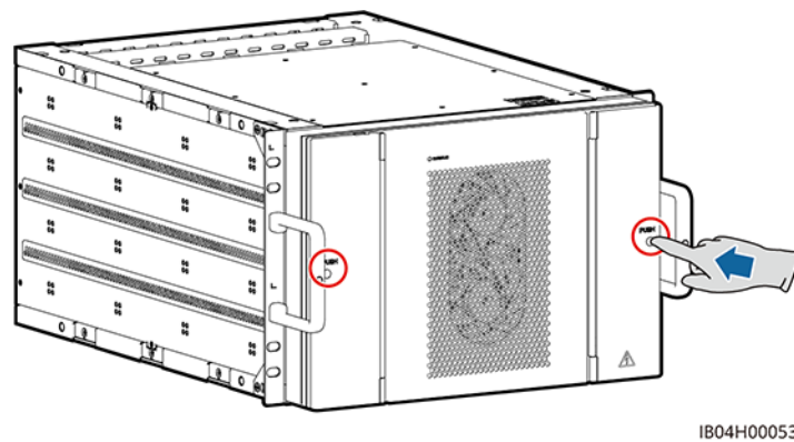
Figure 5-13 Closing the battery pack covers
