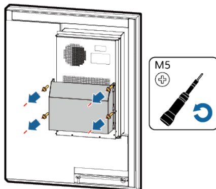
Figure 10-1 Removing the air duct
