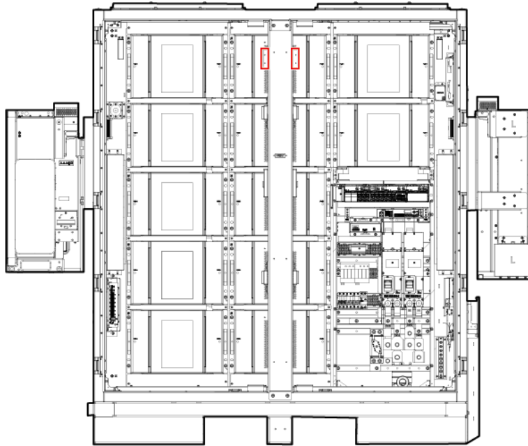
Figure 19-1 Positions of door status sensors
