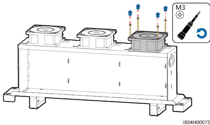
Figure 9-7 Removing the fan
