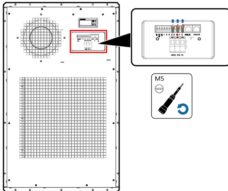
Figure 10-2 Removing air conditioner cables
