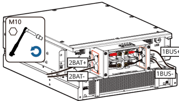
Figure 8-2 Removing the BAT/BUS terminal cables
