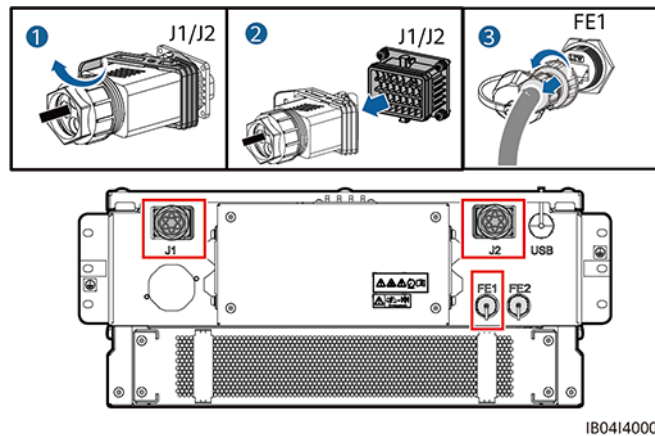
Figure 8-3 Removing the J1 and J2 terminals, and the FE network cable
