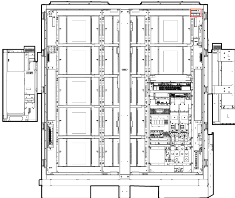
Figure 26-1 Position of the smoke detector
