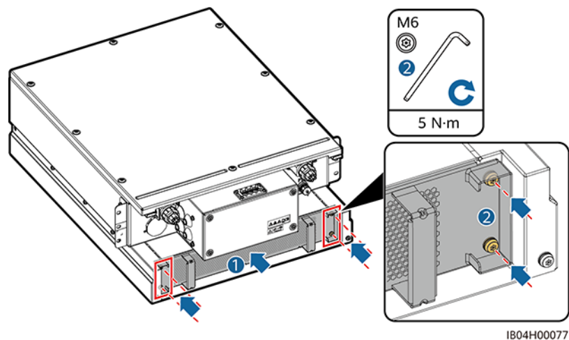
Figure 9-13 Reinstalling the fan tray
