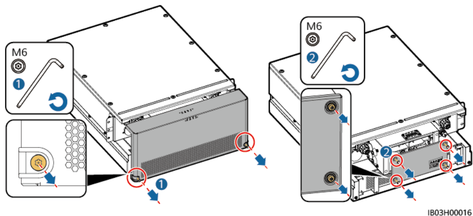
Figure 8-1 Removing covers
