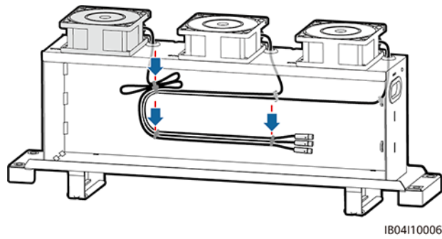
Figure 9-11 Binding the cable of FAN 3
