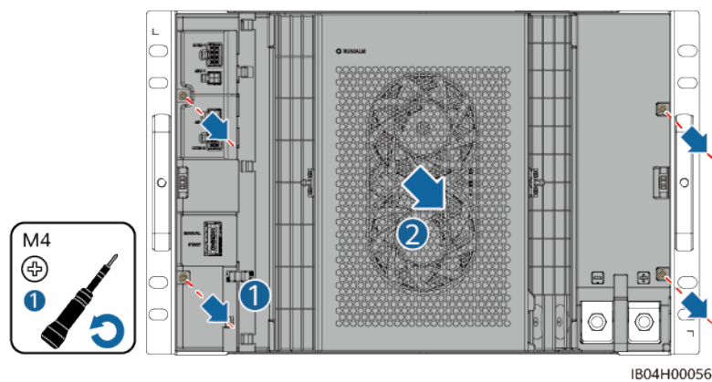
Figure 5-3 Removing the front panel of the battery pack
