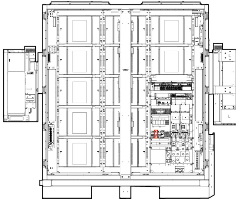
Figure 13-4 Position of the AC main switch
