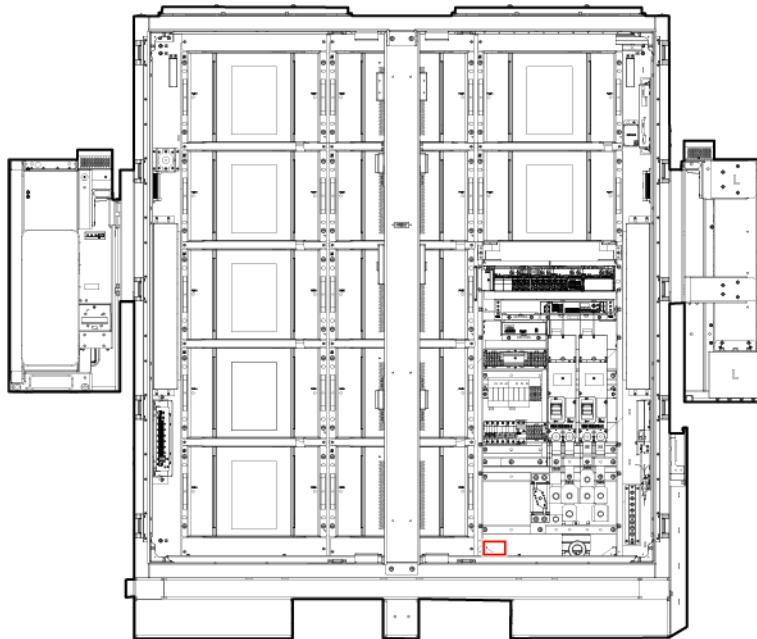
Figure 20-1 Position of the water sensor
