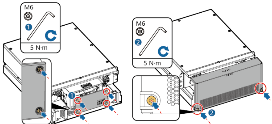
Figure 8-6 Installing covers
