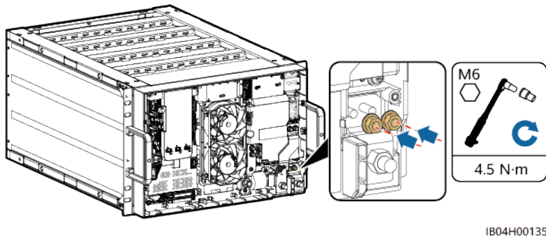
Figure 5-9 Installing the nuts
