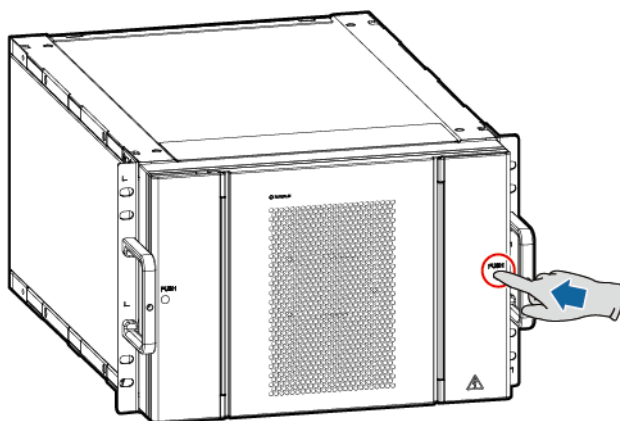
Figure 5-1 Opening the battery pack covers
