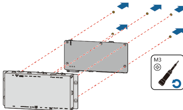
Figure 22-3 Removing the old TCUE control board
