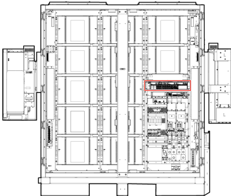
Figure 16-1 Position of the embedded power subrack
