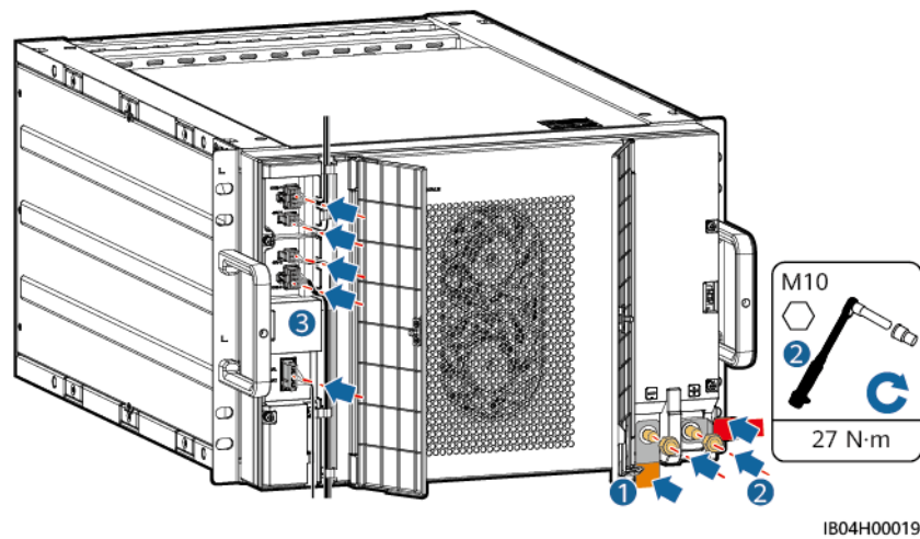
Figure 5-12 Installing copper bars and cables for the battery pack
