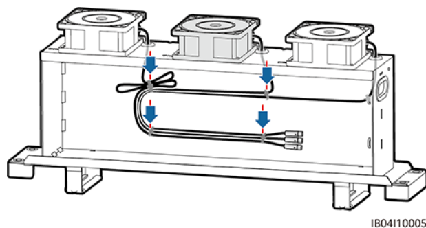
Figure 9-10 Binding the cables of FAN 2
