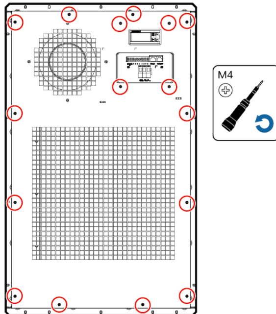
Figure 10-12 Removing the front cover of the air conditioner
