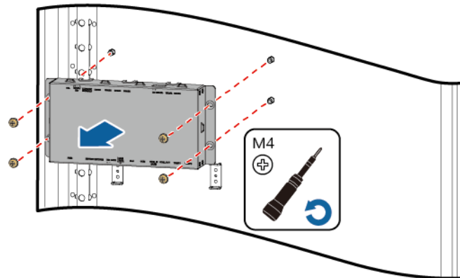
Figure 22-2 Removing the TCUE control box
