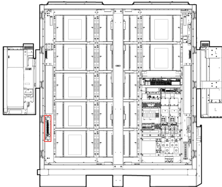
Figure 27-1 Position of the I/O expansion board
