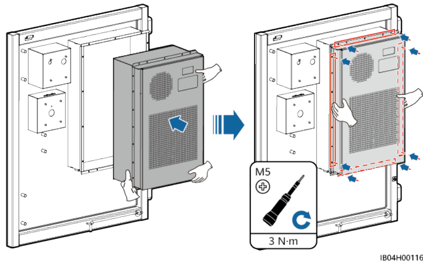
Figure 10-19 Installing a new air conditioner
