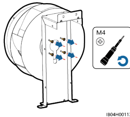
Figure 10-9 Removing the external fan
