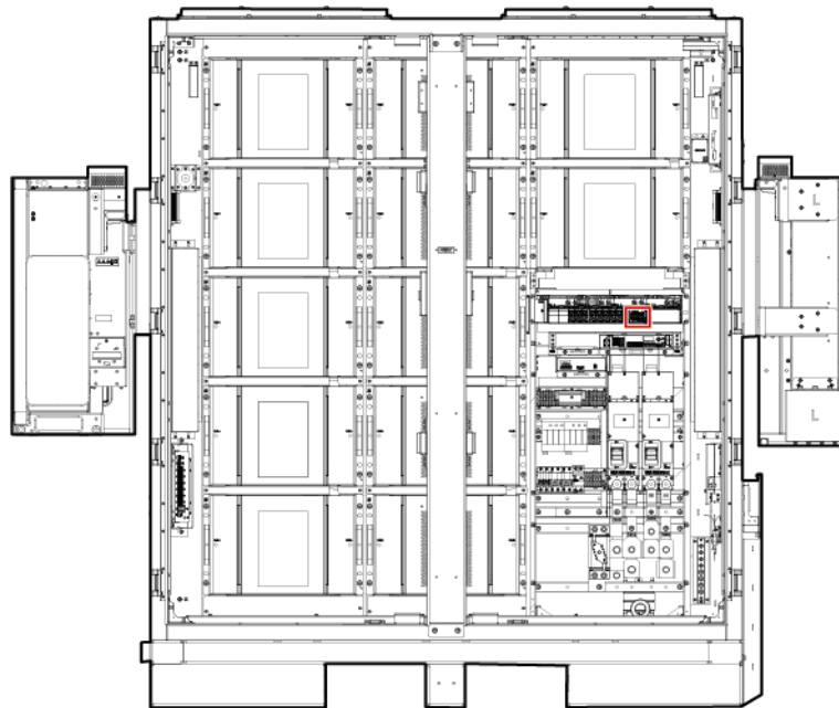
Figure 25-1 Position of the SMU11B
