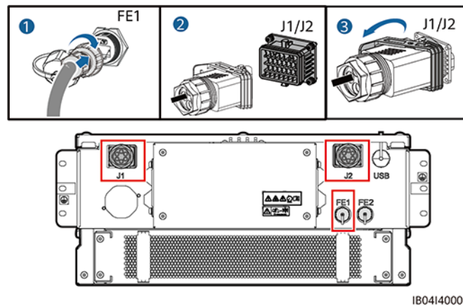
Figure 8-16 Installing cables (part 2)
