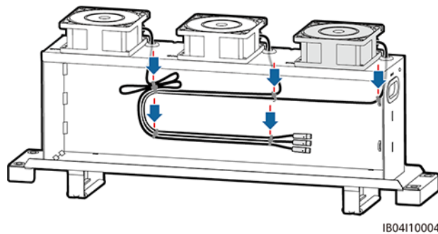
Figure 9-9 Binding the cables of FAN 1
