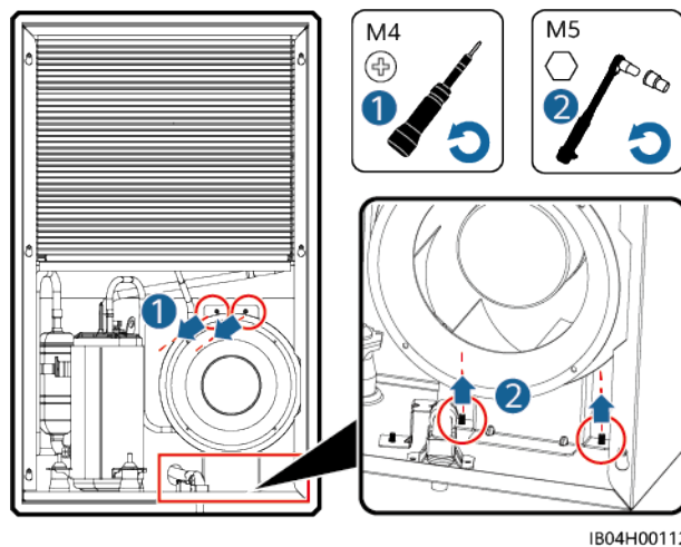
Figure 10-8 Removing the external fan and the fixing plate
