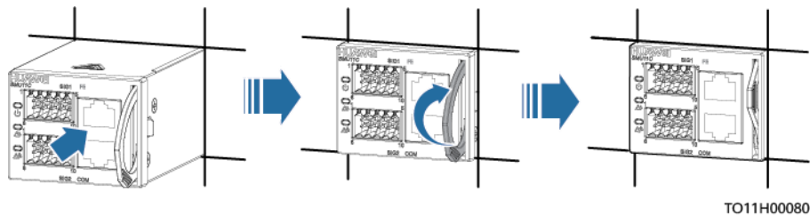
Figure 25-3 Installing the new SMU
