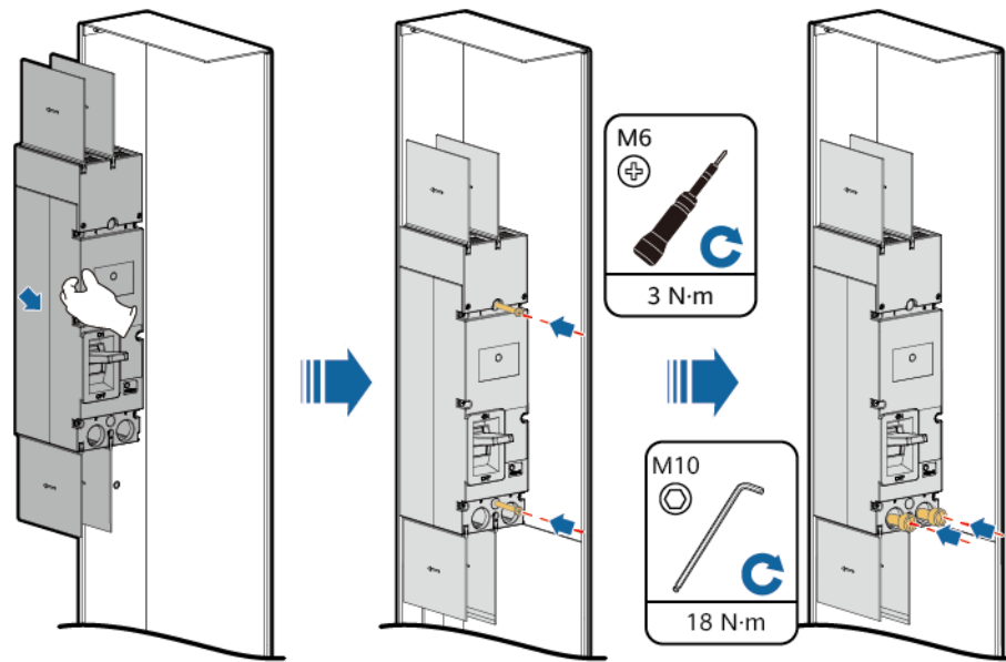
Figure 13-3 Installing a DC switch
