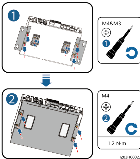
Figure 18-4 Replacing a CMU
