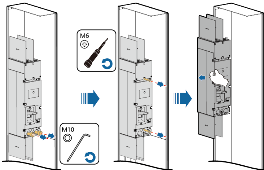
Figure 13-2 Removing the DC switch
