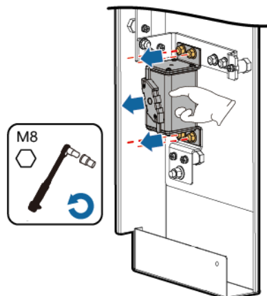
Figure 12-1 Removing the fuse
