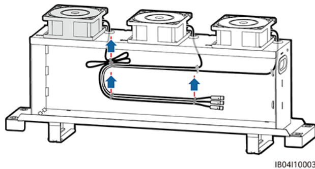
Figure 9-6 Removing the FAN 3 cable ties
