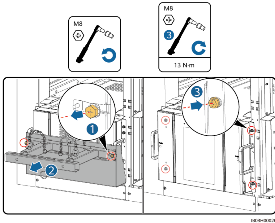
Figure 4-11 Securing the battery pack
