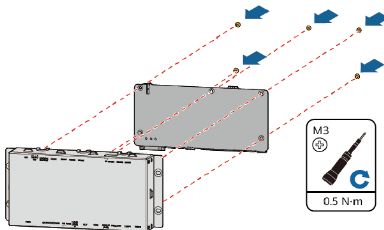
Figure 22-5 Installing the new TCUE control board
