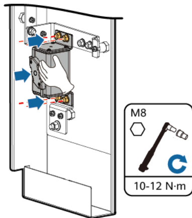
Figure 12-2 Installing a new fuse
