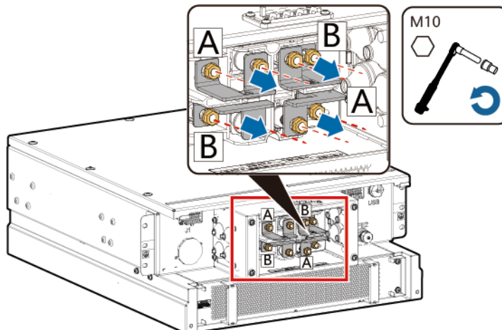
Figure 8-4 Removing short-circuiting copper bars (200 kWh model)
