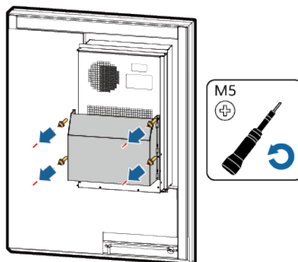
Figure 10-16 Removing the air duct
