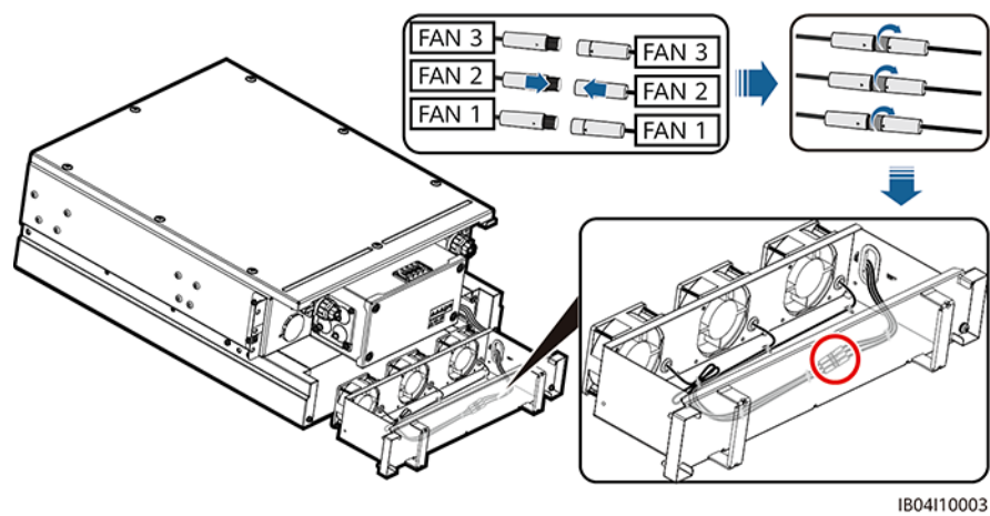
Figure 9-12 Binding cables
